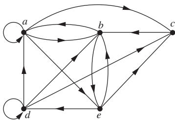
FIGURE 1 A directed graph.
